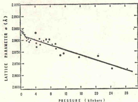
Fig. 1. Lattice parameters of chromium vs. pressure.
